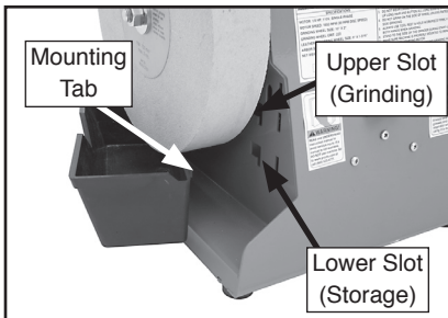
Figure 8. Reservoir mounting positions.
